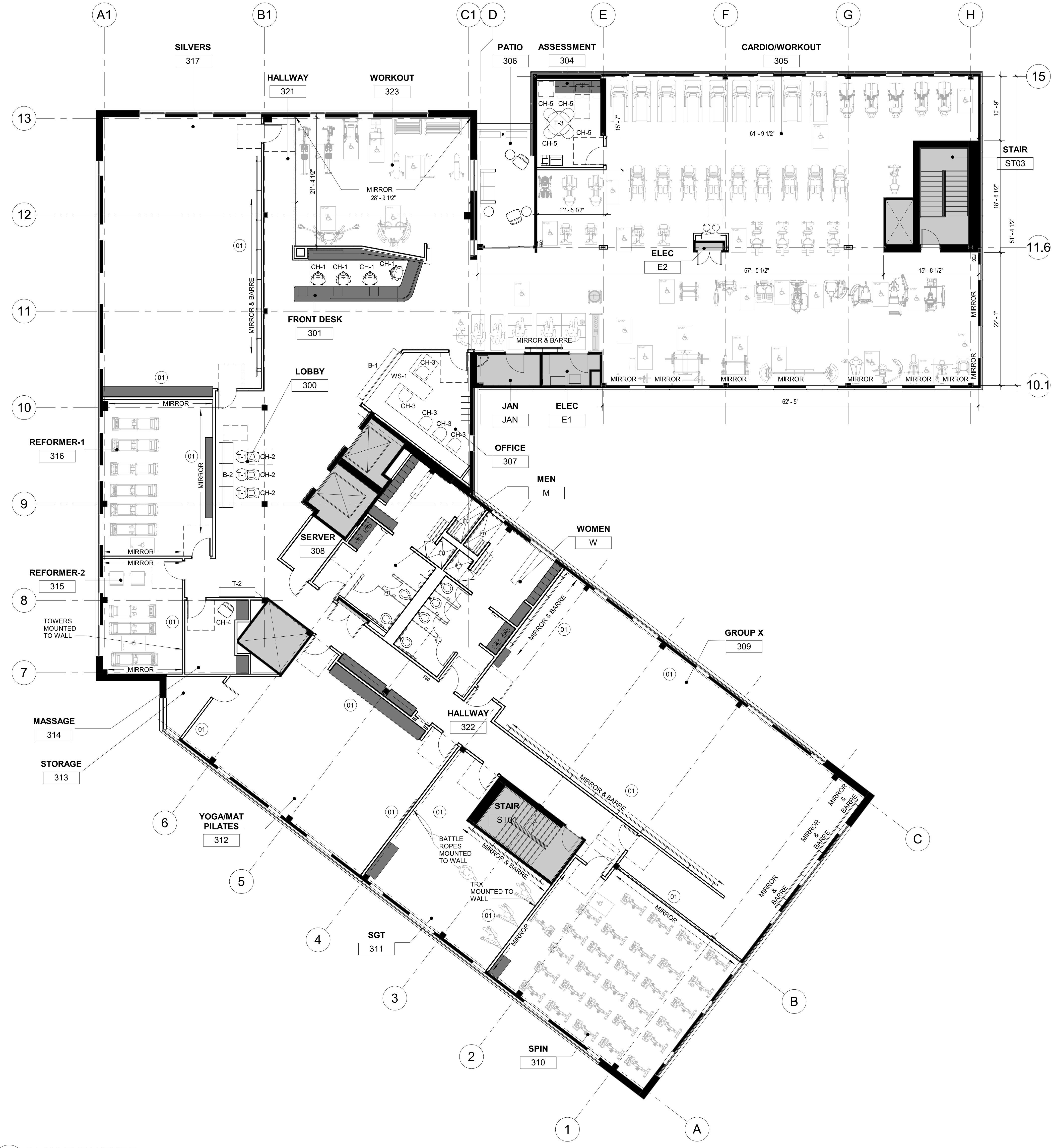
1 PLAN-FURNITURE 1/8" = 1'-0"
